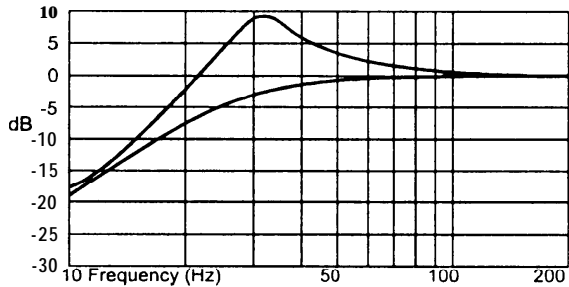
FIG. 2 VARIABLE "Q"
