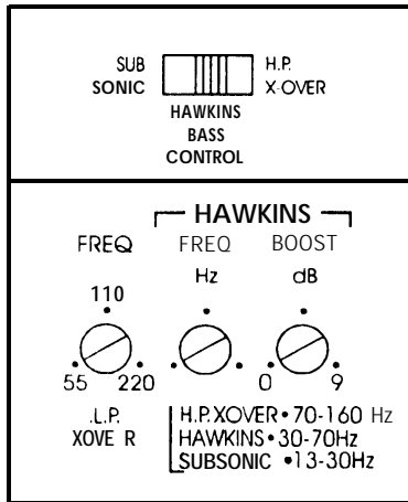
FIG. 1 BASS CONTROL
