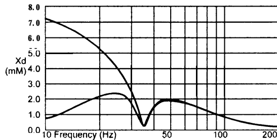
FIG. 5 LIMITED EXCURSION
