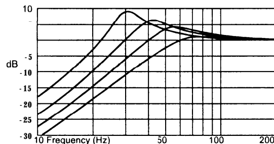
FIG. 6 VARIOUS SETTINGS
