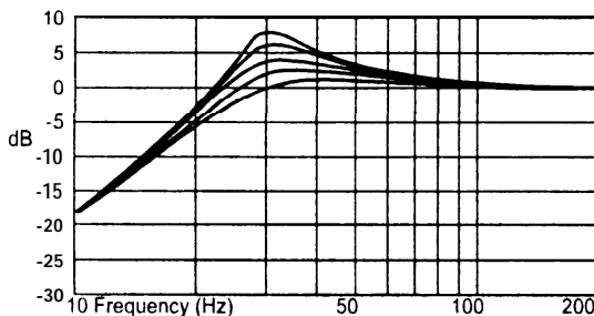
FIG. 4 VARIABLE BOOST
