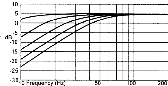
FIG. 3 VARIABLE HIGH PASS
