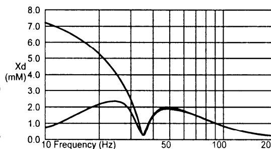
FIG. 3 Limited Excursion
