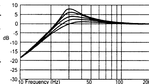
FIG. 2 VARIABLE BOOST
